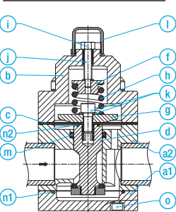
50 mm V82 INSIDE STRUCTURE DIAGRAM
